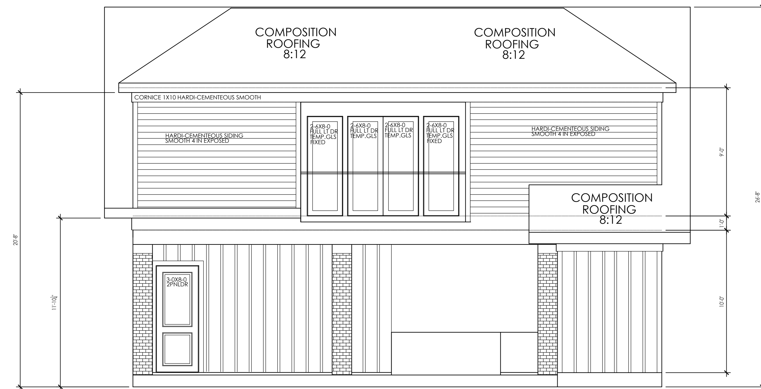
REAR/EAST ELEVATION
